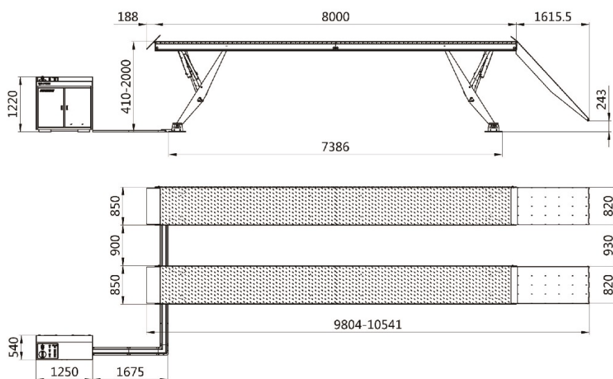
OVERALL DIMENSION
