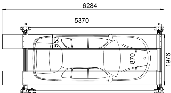
Top Plan View
